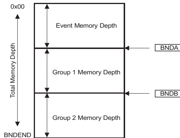
Figure 19-3. FIFO Implementation
