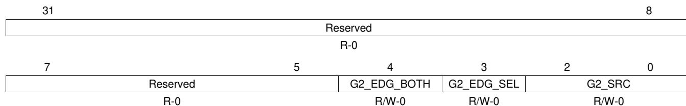
Figure 19-30. ADC Group2 Trigger Source Select Register (ADG2SRC) [offset = 24h]
