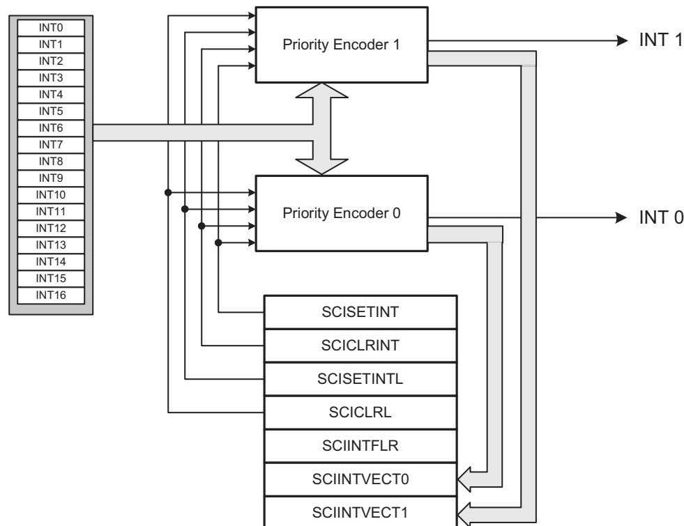
Figure 26-6. General Interrupt Scheme
