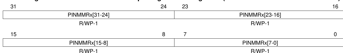
Figure 4-15. PINMMRnn: Pin Multiplexing Control Registers (Address = FFFFEb10h-FFFFE88h)
