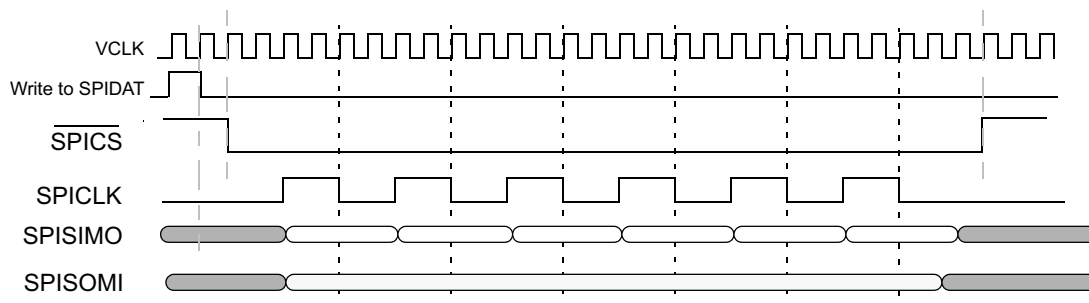
Figure 24-82. SPI/MibSPI Pins During Master Mode 4-pin with \overline{\text{SPICSS}} Configuration
