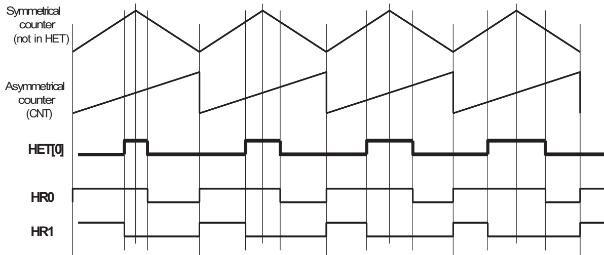
Figure 20-14. Symmetrical PWM with XOR-sharing Output
