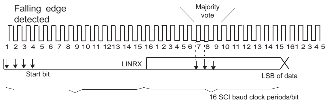
Figure 25-4. Asynchronous Communication Bit Timing
