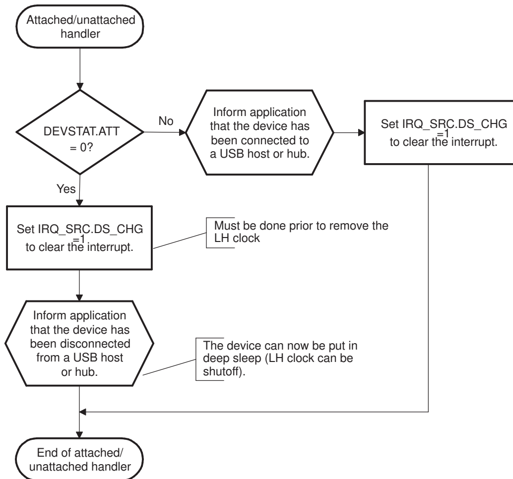
Figure 29-71. Attached/Unattached Handler
