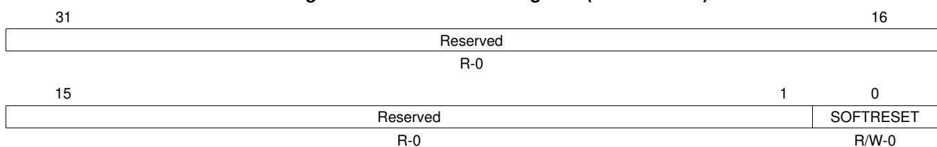
Figure 28-75. Soft Reset Register (SOFTRESET)
