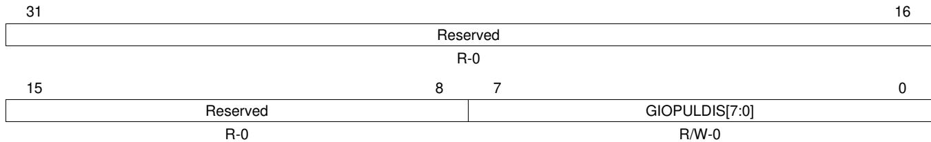
Figure 22-23. GIO Pull Disable Registers (GIOPULDIS[A-B]) [offset = 4Ch, 6Ch]
