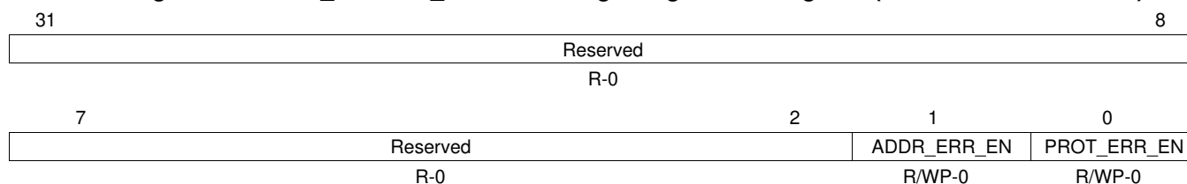
Figure 4-10. ERR_ENABLE_REG: Error Signaling Enable Register (Address = FFFF0AE8h)
