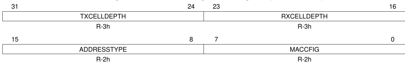
Figure 28-74. MAC Configuration Register (MACCONFIG)
